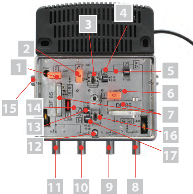
Fig. 2: HV 422-85 Vario amplifier, interior view
